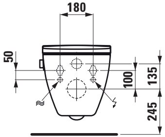
Connection with Laufen installation system LIS CW2
