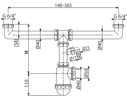
A448: H=195-300 A448P: H=240-300
