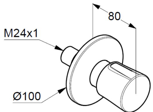
Dimensional drawing
